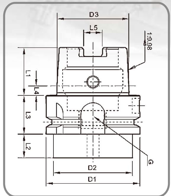
HSK-A100 tool holder
