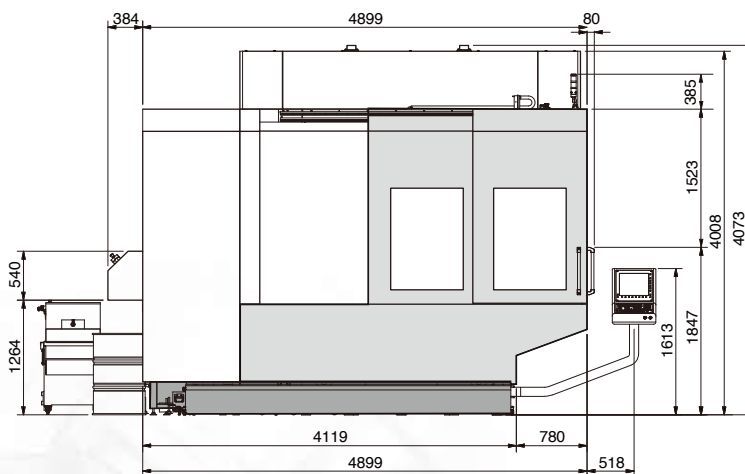
1. FRONT VIEW
