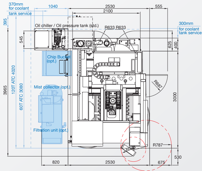
Installation dimension
